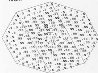
Total SPL with 50 watts.
