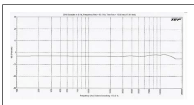
flat (SVT40 mic without cap)
