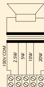
Circuit Diagram
