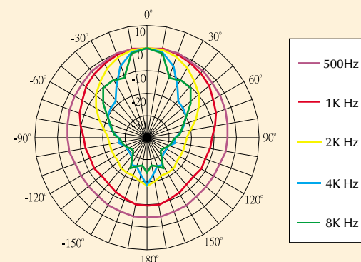
Polar Pattern
