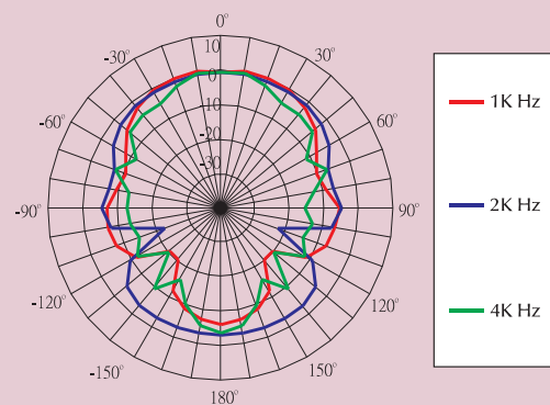
Polar Pattern
