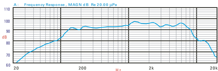
Frequency Response
