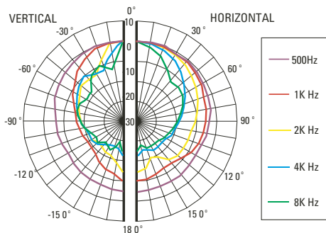
Polar Pattern
